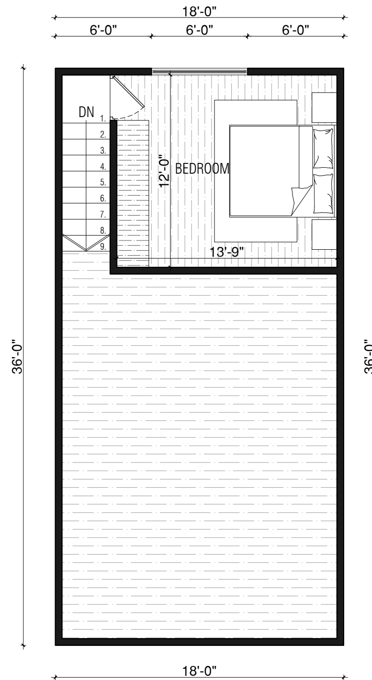
MEZZANINE FLOOR
